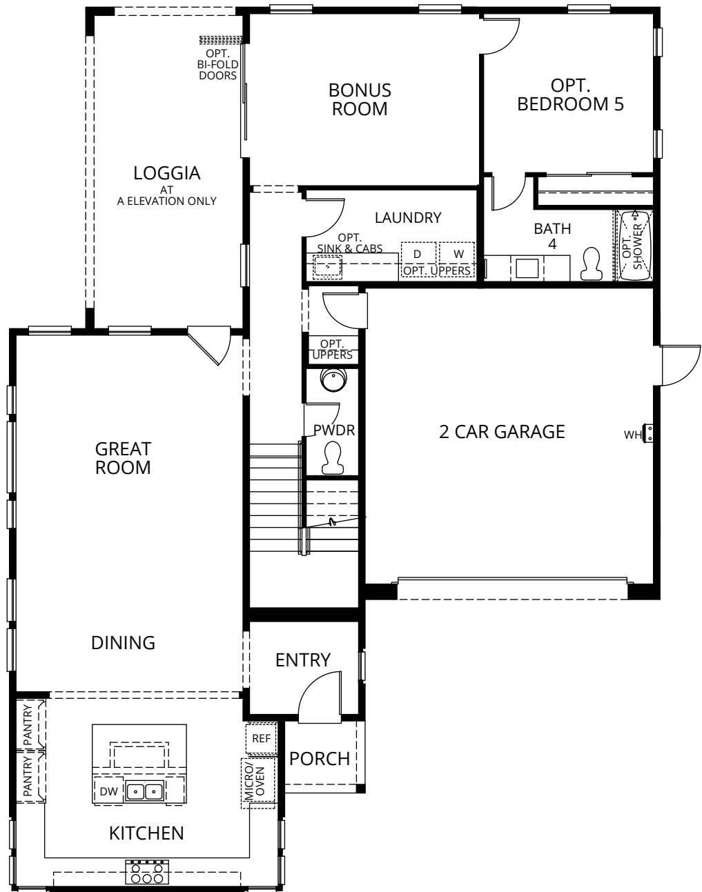
FIRST FLOOR
